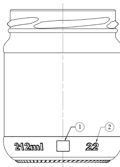
VIEW C SCALE 1 : 1
